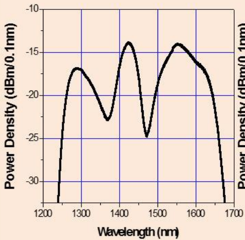
Spectrum Combination of 4 SLEDs (1250-1650 nm)
