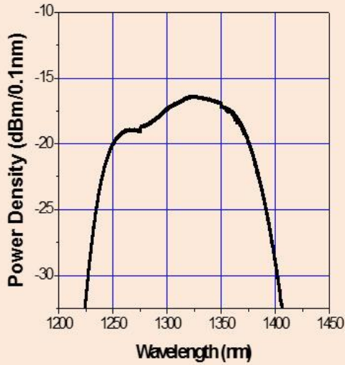
Spectrum Combination of 2 SLEDs (1230-1400 nm)
