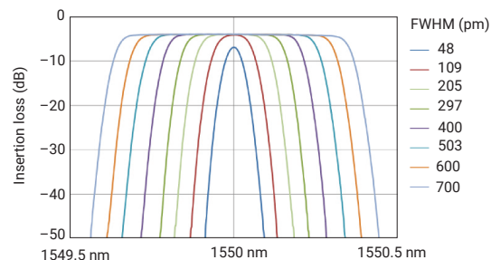
Figure 2. Bandwidth and wavelength tuning
