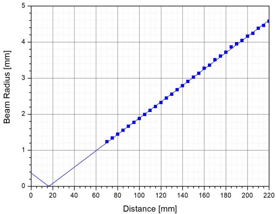
Beam divergence
